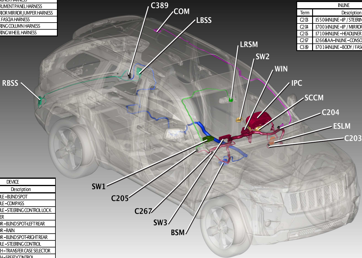
LIN Network Topology
